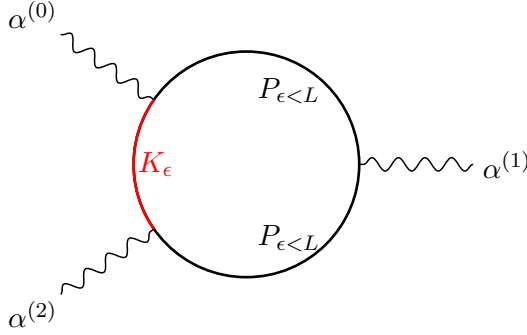
Figure 1: The diagram representing the weight W_{\Gamma,e}(P_{\epsilon < L}, K_\epsilon, I^{\mathfrak{g}}) in the case d = 2 . On the black internal edges we place the propagator P_{\epsilon < L} of the \beta\gamma system. On the red edge labeled by e we place the heat kernel K_\epsilon . The external edges are labeled by elements \alpha^{(i)} \in \Omega_c^{0,*}(\mathbb{C}^2) .
