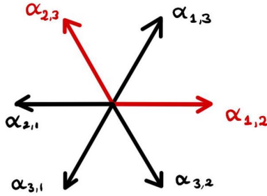
FIGURE 4. Root system of GL_3 with a choice of basis \Delta = \{\alpha_{1,2}, \alpha_{2,3}\} in red
