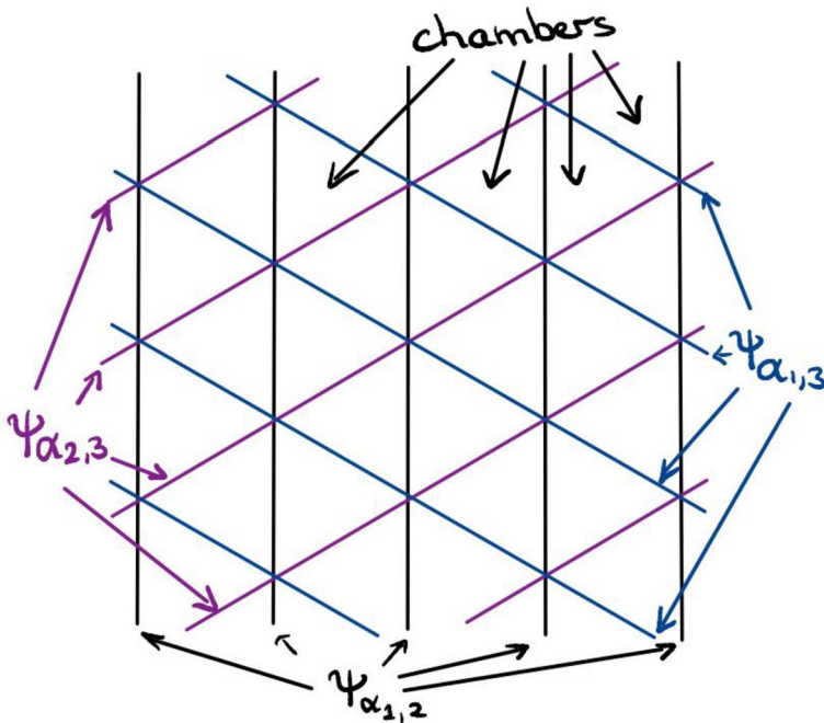
FIGURE 5. Excerpt of an apartment for SL_3 with hyperplanes
