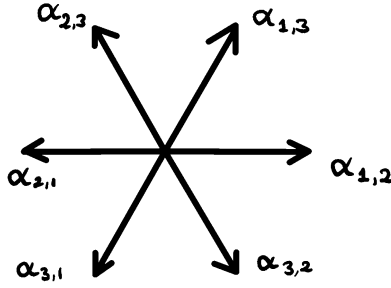
FIGURE 2. Root system of GL_3
