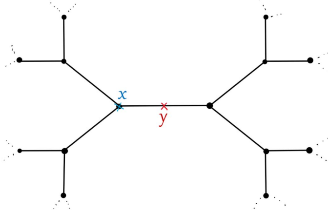
FIGURE 1. Bruhat–Tits building for \mathrm{SL}_2(\mathbb{Q}_2) .
