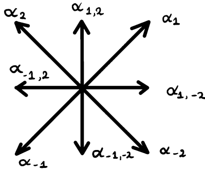
FIGURE 3. Root system of Sp_4
