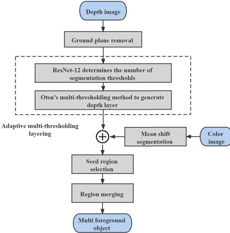
Figure 1: The proposed method.
