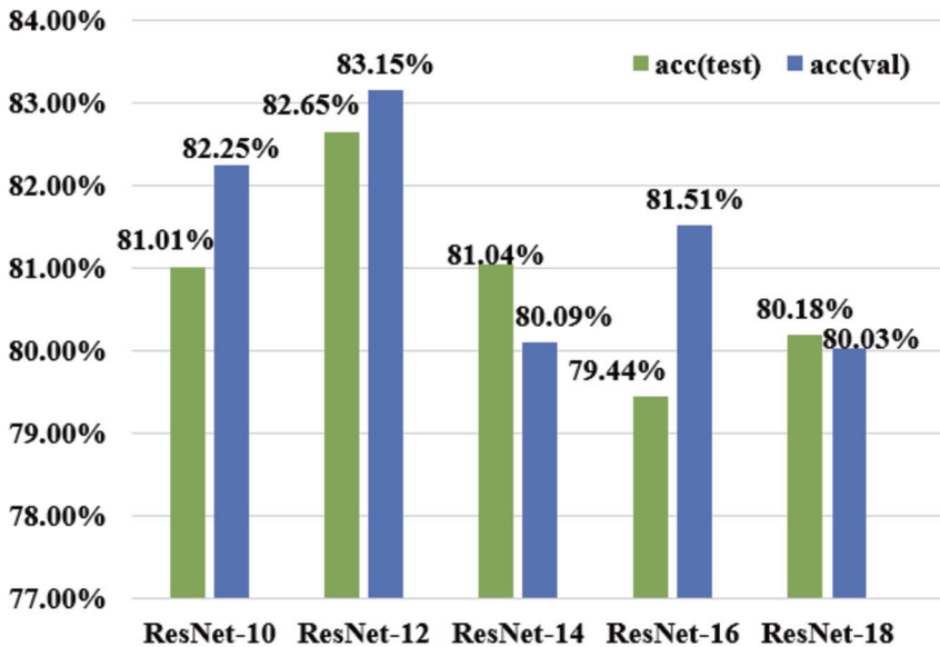
Figure 11: Experimental results of ResNets.
