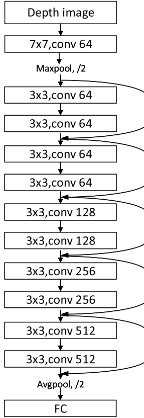
Figure 6: RestNet12 network structure diagram.
