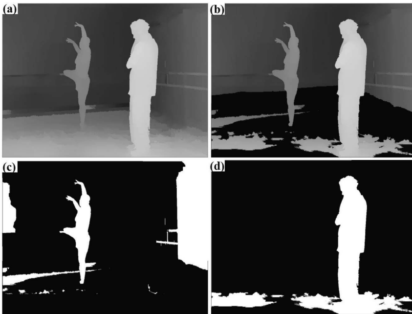
Figure 7: The result image of adaptive segmentation. (a) Depth image; (b) Depth image after removing the ground plane; (c) First layer image; (d) Second layer image.
