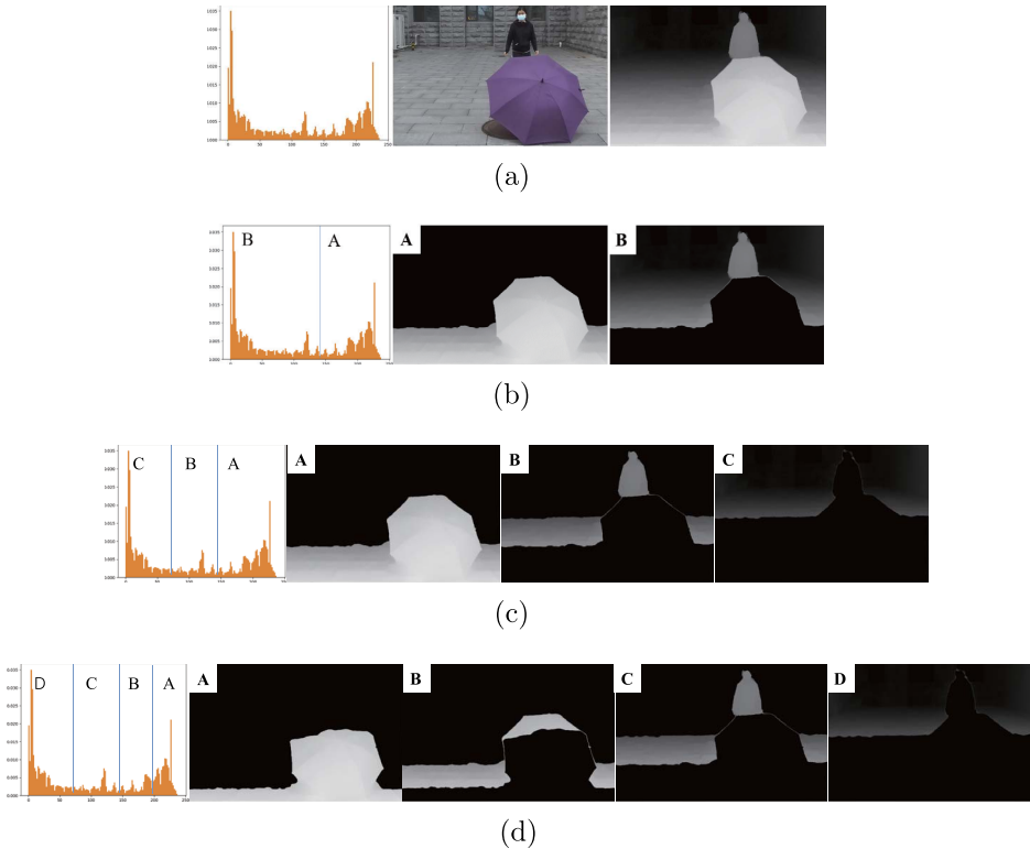
Figure 4: Multiple depth layers of depth image obtained by extended Otsu’s multi-thresholding method [8]. (a) Depth image and its histogram; (b) Two depth layers generated with one threshold; (c) Three depth layers with two thresholds; (d) Four depth layers with three thresholds.
