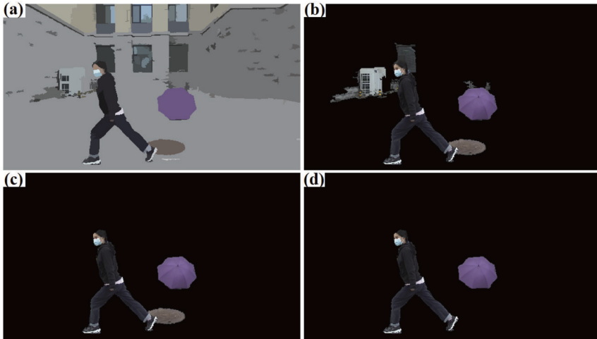
Figure 10: Comparison of region merging results. (a) RGB image after mean-shift segmentation; (b) merged result using area constraint only; (c) merged result using area constraint and depth layering constraint (the depth image does not remove the road surface); (d) our result.
