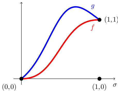
FIG. 2.1. Diagrams of the flux \sigma \mapsto f(\sigma, \gamma, \kappa) and of the function \sigma \mapsto g(\sigma, \gamma, \kappa) = f(\sigma, \gamma, \kappa) / \sigma for fixed values of \gamma and \kappa .
