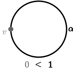
Figure 1: A stratified circle, S^1 \rightarrow [1] as in Example 2.4, where v \mapsto 0 and \alpha \mapsto 1 .
