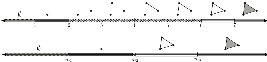
Figure 3: An example of the map C . The relevant interval for the point, e.g., m_2 is [2, 7) , since the image of each simplex added in that interval under the filter function f is m_2 . Then [2, 6) is mapped to m_2 and [6, 7) is mapped to [m_2, m_3) .
