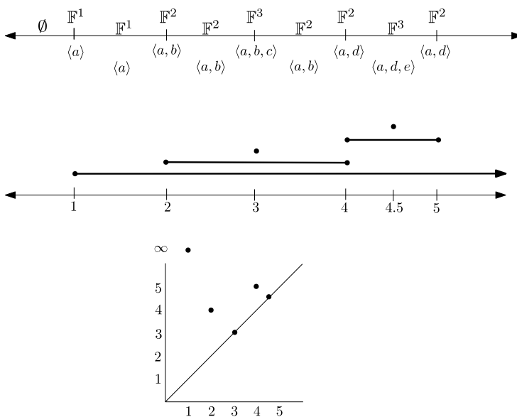
Figure 4: The result of applying \delta to the cosheaf shown on the top of the figure is the persistence diagram shown on the bottom. In the middle, we have drawn the associated barcode. In the spirit of [10], we have shown all bars as closed intervals to emphasize that they do not necessarily arise from a monotone filtration. Note the presence of length-zero barcodes and on-diagonal points, corresponding to indecomposable elements with a single vector space.
