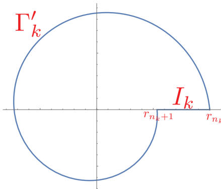
FIG. 2. The curve \Gamma_k = \Gamma'_k \cup I_k .
