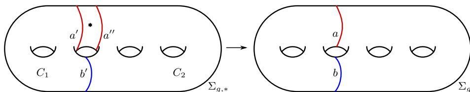
Figure 3: The canonical reduction system for \sigma((T_a T_b^{-1})^k) . Since the curves must be disjoint, there can be at most two curves a', a'' (resp. b', b'' ) that are unmarked-isotopic to a (resp. b ), and moreover there can be at most three total curves. Without loss of generality we eliminate b'' . We further note that following Step 2 we only know that the canonical reduction system is nonempty; prior to Step 3 it is possible that one or more of a', a'', b' does not appear.
