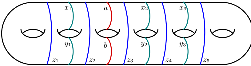
Figure 2: The g - 2 bounding pair maps T_a T_b^{-1} and T_{x_i} T_{y_i}^{-1} , and the g - 1 separating twists T_{z_i} , illustrated for g = 6 . Altogether this determines a copy of \mathbb{Z}^{2g-3} centralizing (T_a T_b^{-1})^k .
