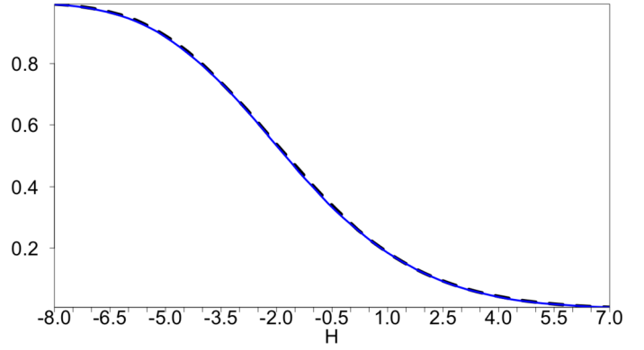
Figure 1. Empirical probabilities of reaching the barrier H (dashed black) and approximation (3.24) (solid blue): A = 1 , M/l_1 = 4 with l_0 = 25 and l_1 = 50 .
