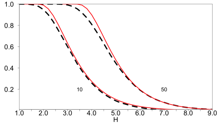
Figure 6. Empirical probabilities of reaching the barrier H (dashed black) and corresponding versions of approximation (3.27) (solid red): A = 1 , m/l_1 = 5 with (a) l_1 = 10 and (b) l_1 = 50 .
