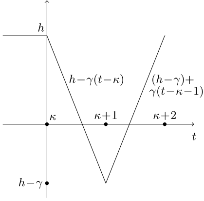
Figure 8. Barrier h - Q(t; \gamma, \kappa) for \lambda = 1 .
