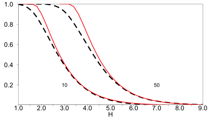
Figure 5. Empirical probabilities of reaching the barrier H (dashed black) and corresponding versions of approximation (3.27) (solid red): A = 1 , m/l_1 = 10 with l_1 = 10 and (b) l_1 = 50 .
