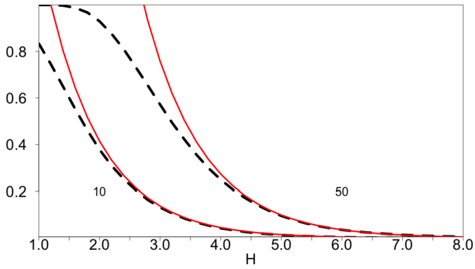
Figure 3. Empirical probabilities of reaching the barrier H (dashed black) and corresponding versions of approximation (3.27) (solid red): A = 1 , m/l_1 = 1 with (a) l_1 = 10 and (b) l_1 = 50 .
