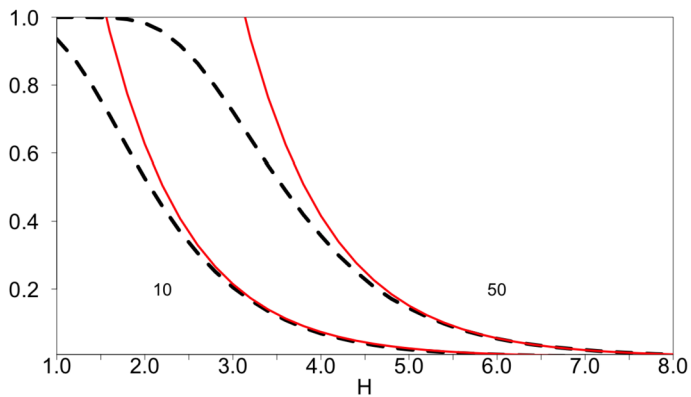
Figure 4. Empirical probabilities of reaching the barrier H (dashed black) and corresponding versions of approximation (3.27) (solid red): A = 1 , m/l_1 = 2 with l_1 = 10 and (b) l_1 = 50 .
