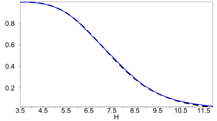
Figure 2. Empirical probabilities of reaching the barrier H (dashed black) and approximation (3.24) (solid blue): A = 0.5 , M/l_1 = 25 with l_0 = 10 and l_1 = 20 .
